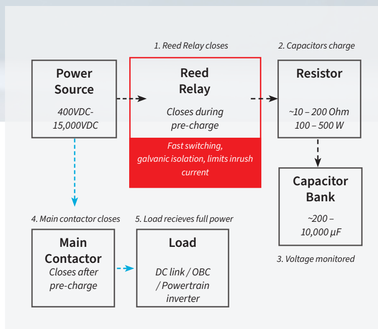
Figure 1. The pre-charge circuit sequence.
