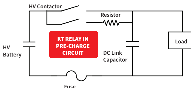
Figure 2. KT Series Reed Relay in the pre-charge circuit.
