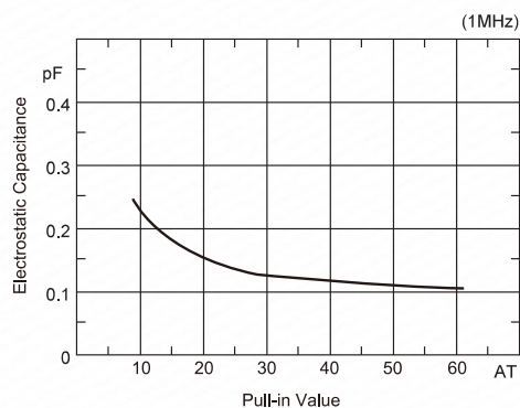
Electrostatic capacitance
