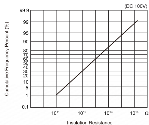
Insulation resistance
