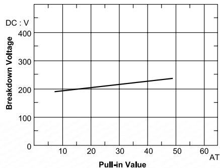
Breakdown Voltage
