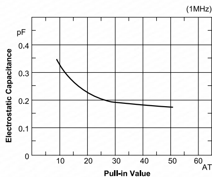
Electrostatic Capacitance
