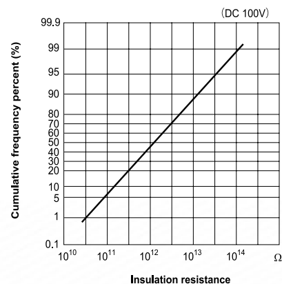
Insulation Resistance
