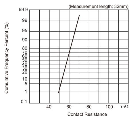
Contact resistance
