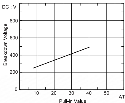
Breakdown voltage
