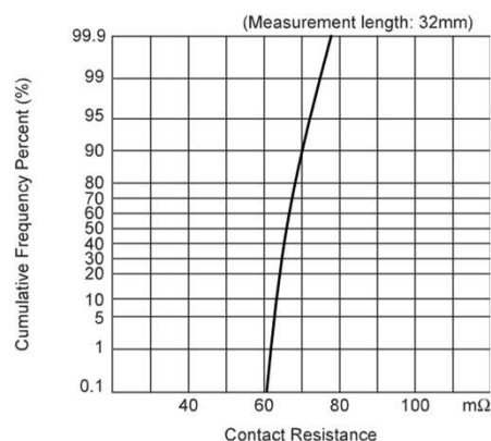
Contact resistance
