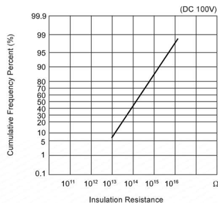
Insulation resistance
