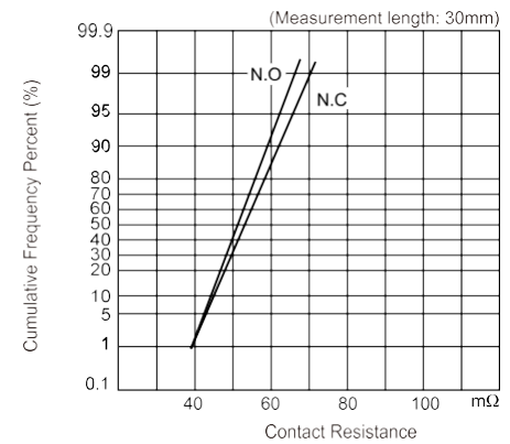
Contact resistance
