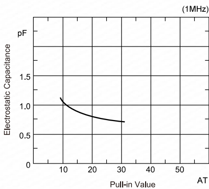
Electrostatic capacitance
